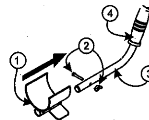
Figure 1 - The armrest and upper shaft assembly
