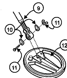
Figure 2 - The coil and lower shaft assembly
